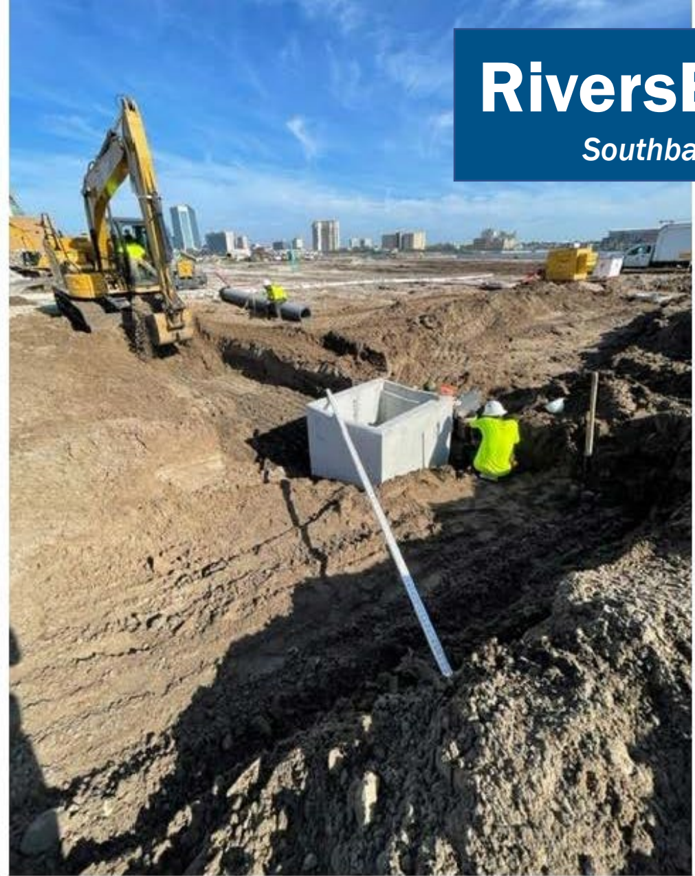
Installing 15" storm drain and installing structure ST-51 on Health Walk Way.
