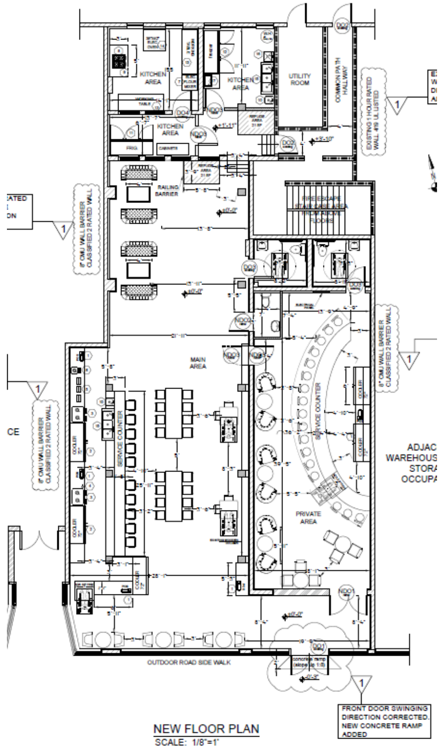
Figure 2 Floor Plan
